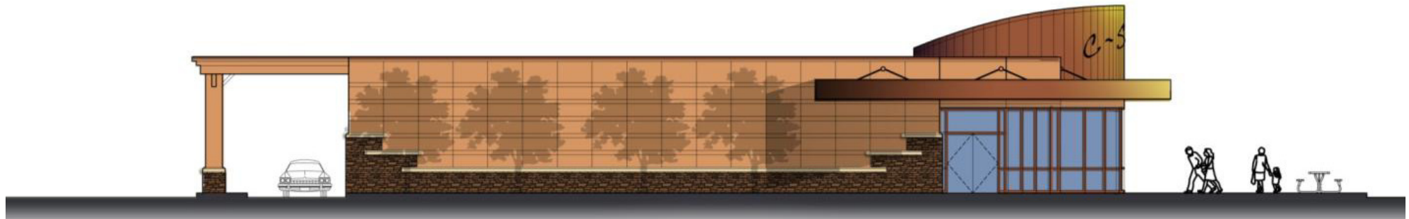
SIDE ELEVATION
